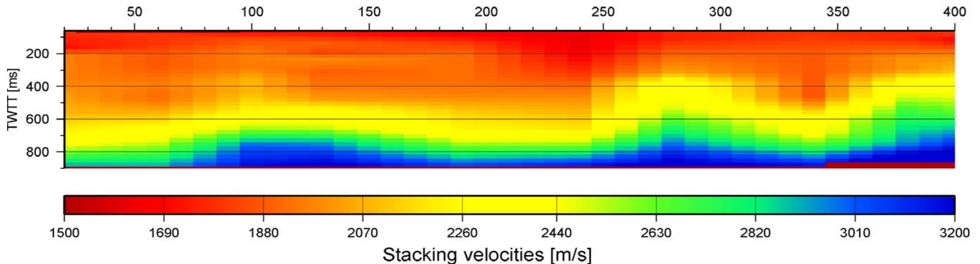
Stacking velocities
