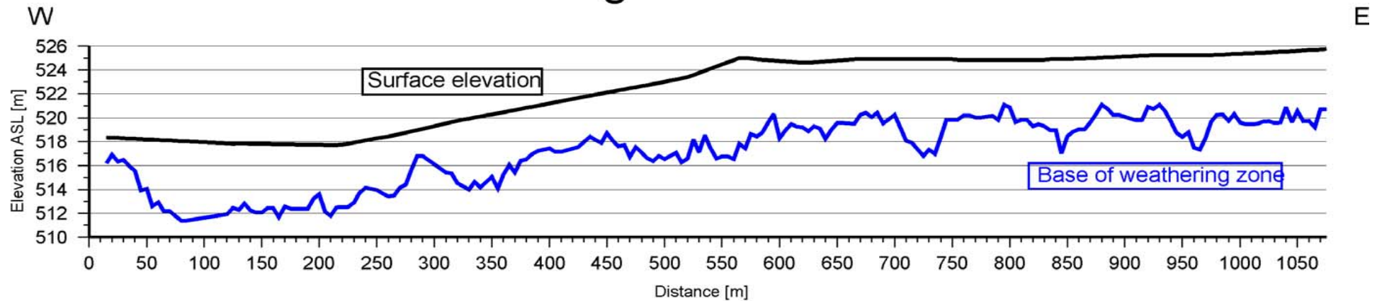
Base of weathering from refraction travel times
