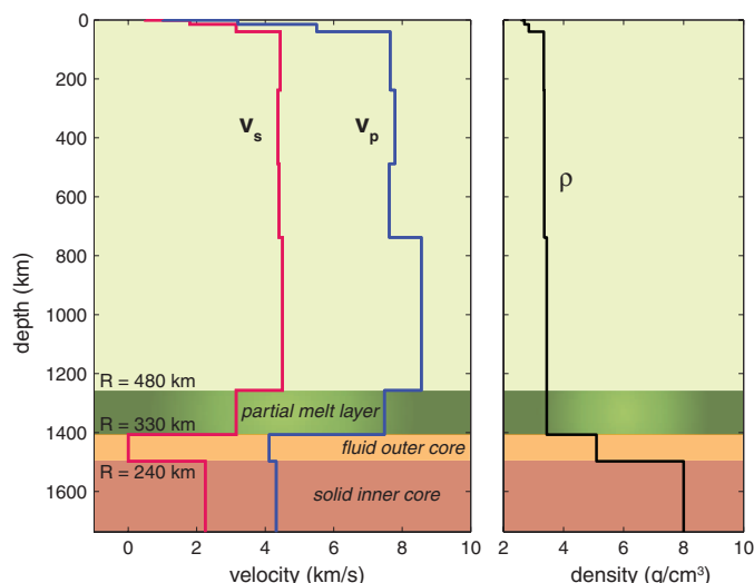
Fig. 3. Preferred velocity ( v ) and density ( \rho ) models. Structure shallower than 1000 km is derived from previous studies (7, 8), whereas that within the core is derived from the elasticity of iron alloys (16, 21, 26).
