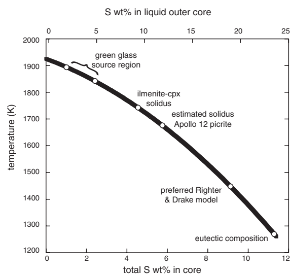
Fig. 4. Tradeoff between the sulfur content of the lunar core and the liquidus temperature. The inner core is assumed to be pure iron, in accord with the eutectic behavior of the Fe-FeS system. Available solidus temperatures at lunar CMB pressures of anhydrous compositions relevant to the overlying partially molten zone, such as the Apollo 12 12009 picrite (22), ilmenite-clinopyroxene cumulates (23), and the green glass source region (24), are also shown, as is an estimate of the sulfur composition of the lunar core derived from siderophile element abundances (27). The phase diagram for the Fe-S system at 5 GPa is interpolated between the ambient-pressure phase diagram, the results of (28) at 3 GPa, and those of (29)
