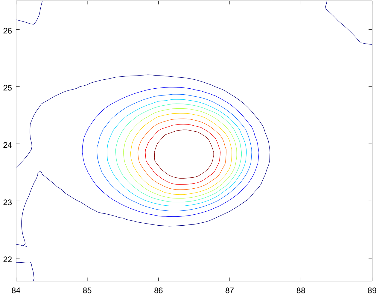
chi at 1Hz from 0.009741 to 0.016006
