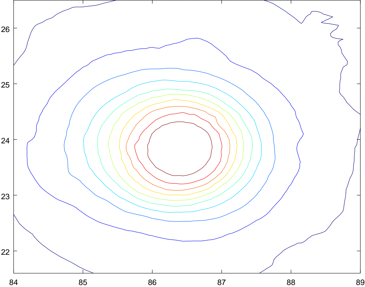
site chi at 14Hz from -0.001943 to -0.000291
